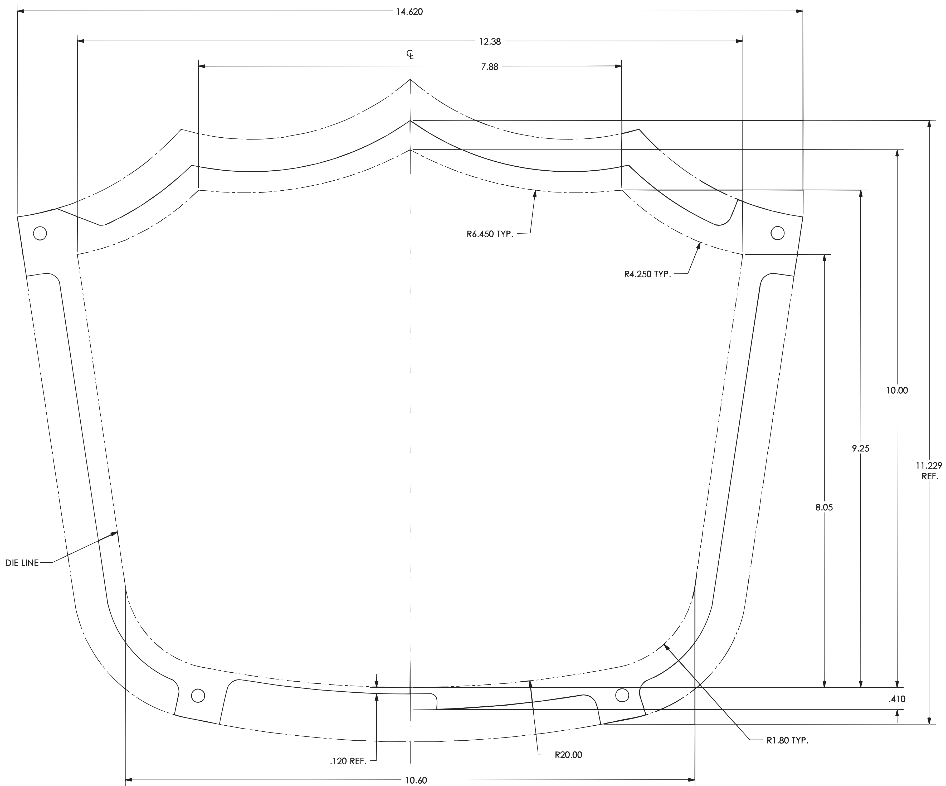
FRONT VIEW
