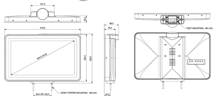
Technical Drawings
