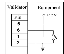
Relay Contact
