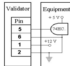
CMOS Logic
