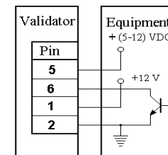
Open Collector
