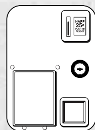
42-7199-00 Upper Door Assembly 1 Coin Entry Validator Cutout with Blanking Plate for use with Mars (300 & 500 Bill Capacity) or Ardac (250 Bill Capacity)
