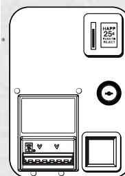
42-7197-00 Upper Door Assembly 1 Coin Entry With Mars AE2411-U5E ($1, $5) Validator (500 Bill Capacity)
