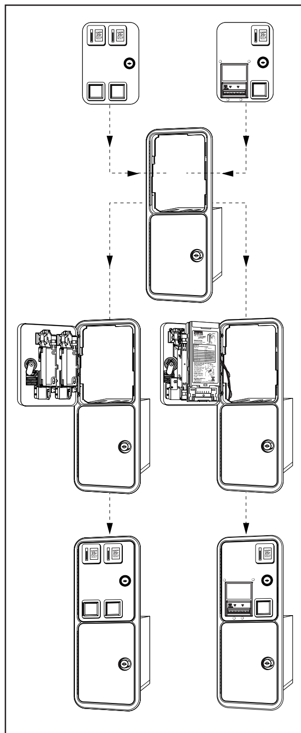
42-7270-00 Upper Door Assembly 1 Coin Entry With Ardac USA3 (88x5033) ($1, $5) Validator (250 Bill Capacity)
