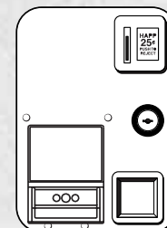
42-7270-00 Upper Door Assembly 1 Coin Entry With Ardac USA3 (88x5033) ($1, $5) Validator (250 Bill Capacity)
