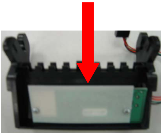
Platform BEG with PCB heat shield
