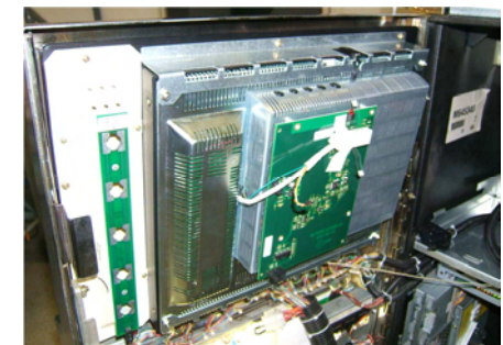
CPA2226, CPA2227- Door Mount Version
